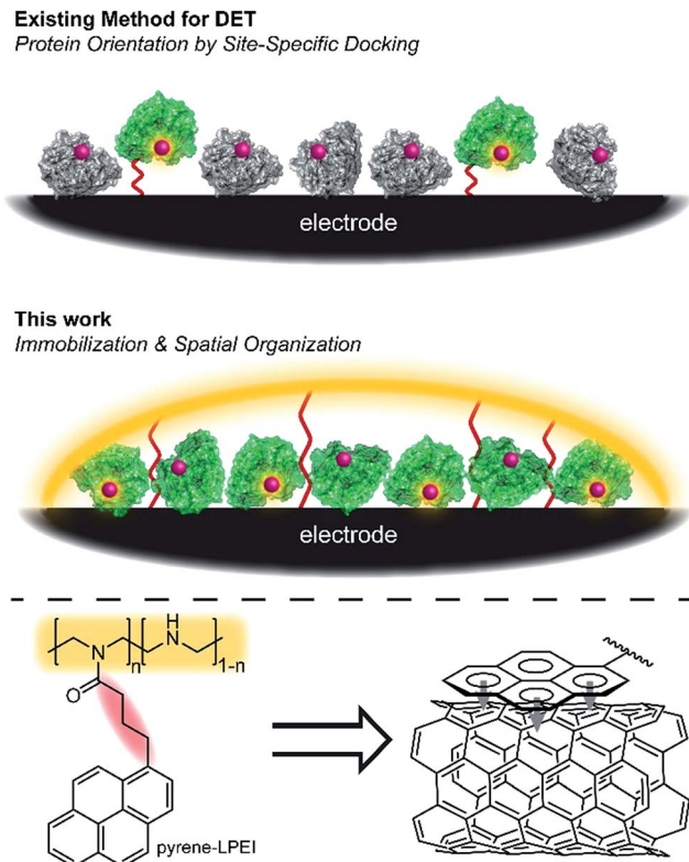
Fig. 1 Scheme depicting the docking approach as compared to the hydrogel immobilization approach described here. Active redox protein is depicted in green, while inactive/denatured redox protein is depicted as grey.
