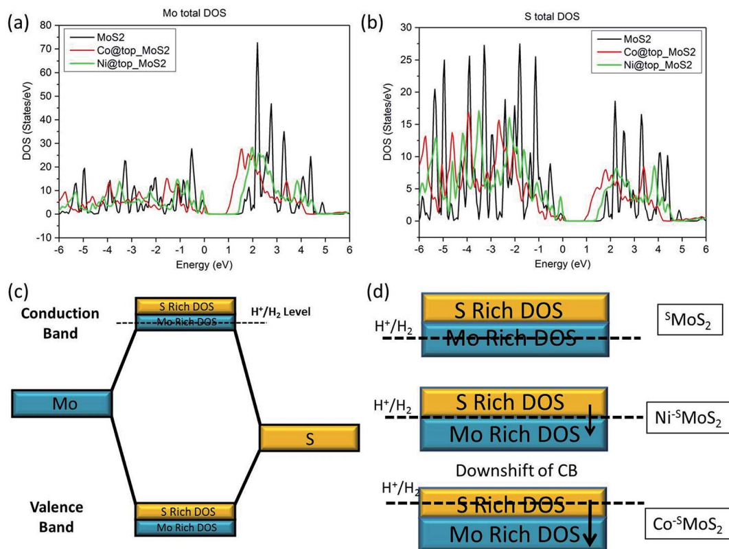
Fig. 7 Calculated Density of States (DoS) of (a) Mo and (b) S in S MoS 2 , Co- S MoS 2 and Ni- S MoS 2 (c) simplified molecular orbital diagram of MoS 2 (d) downshift of the conduction band (CB) upon addition of a single Co and Ni metal atom at the Mo atop site, respectively.
