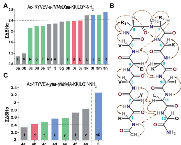
Fig. 4 (A) \Sigma\text{CSD} of the primary library with L-amino acid substitutions (Xaa) at the i+2 site. (B) The characteristic NOEs, where the thick arrows denote strong (1.8–2.1 Å), the thin arrows denote medium (2.2–2.5 Å) and the broken arrows denote weak (>2.6 Å) NOEs. (C) \Sigma\text{CSD} of the secondary library with i+1 substitutions (yaa) along with 5 derived from the combination of 4g and 3n. All the NMR measurements were done in acetate buffer (pH 3.8) at 25 °C.
