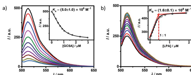
Fig. 1 (a) Direct fluorescence titration of FI (1.0 \mu\text{M} ) with GC5A (up to 3.0 \mu\text{M} ), \lambda_{\text{ex}} = 500 \text{ nm} . (Inset) the associated titration curve at \lambda_{\text{em}} = 513 \text{ nm} and the fit according to a 1 : 1 binding stoichiometry. (b) Competitive titration of GC5A·FI (0.4/0.5 \mu\text{M} ) with LPA (up to 1.9 \mu\text{M} ). (Inset) fit of the titration data to a 1 : 1 competitive binding model. All experiments are in HEPES buffer (10 mM, pH = 7.4) at 25 °C.
