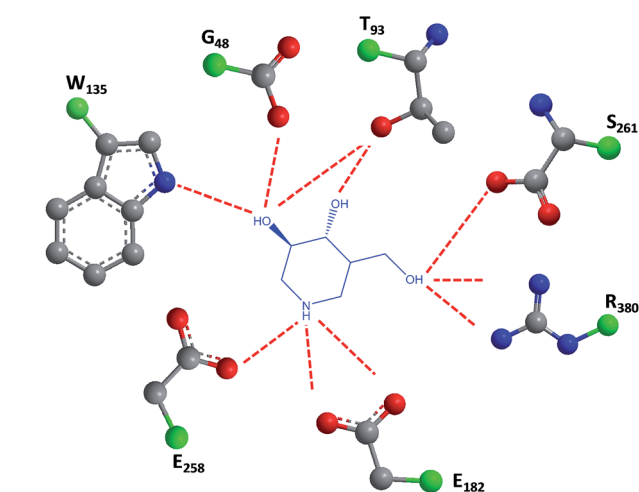
Fig. 6 Schematic representation of hydrogen bond interactions (red dashed lines) between GALC and isofagomine (7). Data from Protein Data bank ( https://www.rcsb.org/pdb ) and ref. 1.
