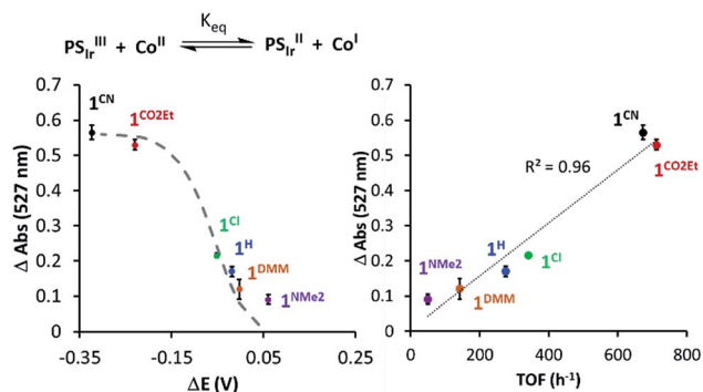
Fig. 7 (Left) The 527 nm absorbance decay upon addition of 1 R vs. \Delta E_{1/2}(\text{PSIr}^+/\text{PSIr}) - E_{1/2}(\text{Co}^{\text{II/I}}) . (Right) 527 nm absorbance of PS Ir decay upon addition of 1 R vs. TOF (h -1 ) (initial rate at 10% conversion of H 2 evolution). The dashed grey line refers to the theoretical values predicted from Nernst equation (see Section ESI 6.1†).
