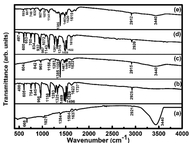
Fig. 4 FTIR spectra of (a) SWCNTs-COOH; (b) F_{16}CoPc ; (c) S_1 ; (d) F_{16}ZnPc and (e) S_2 hybrid.
