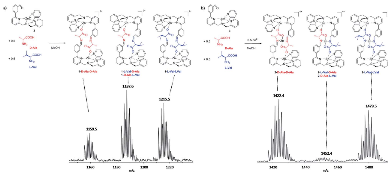
Fig. 3 ESI-MS signals corresponding to (a) 1-D-Ala-D-Ala , 1-L-Val-D-Ala and 1-D-Val-L-Ala , 1-L-Val-L-Val ; (b) 2-D-Ala-D-Ala , 2-L-Val-D-Ala and 2-D-Val-L-Ala , 2-L-Val-L-Val . The cluster in the ESI-MS spectra are referred to the mono-charged species in which the counteranions are perchlorate.
