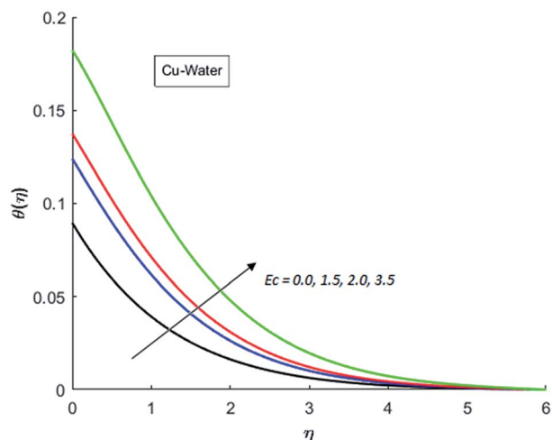
Fig. 15 Temperature curves for various value of Ec when M = 0.5 , Pr = 0.3 , Gr = 5 , Nr = 0.2 and \lambda = 1 .
