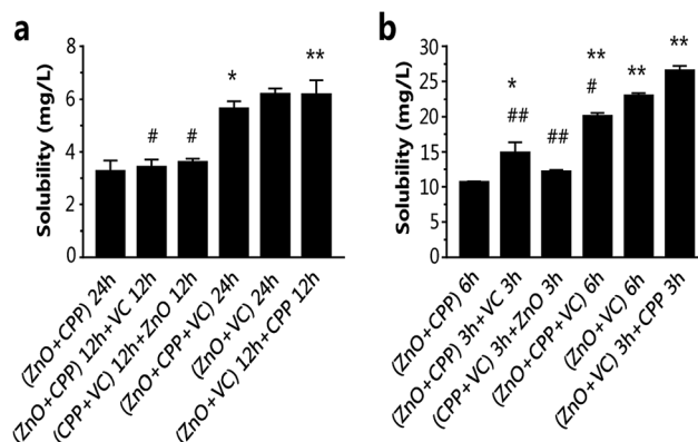
Fig. 6 Solubility of ZnO NPs in different systems at different time. (a) Solubility of 15 mg L -1 ZnO NPs at 24 h; (b) solubility of 120 mg L -1 ZnO NPs at 6 h. Data are presented as the mean \pm S.D. * P < 0.05 compared with the group of ZnO NPs plus CPP. ** P < 0.01 compared with the group of ZnO NPs plus CPP. # p < 0.05 compared with the group of ZnO NPs plus VC. ## p < 0.01 compared with the group of ZnO NPs plus VC.
