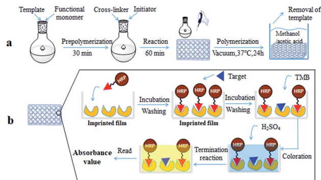
Fig. 1 Preparation of the molecularly imprinted film on the surface of the 96-well plate (a); direct competitive BELISA procedure (b).
