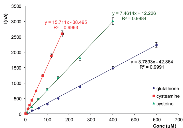
Fig. 3 The calibration curves obtained with screen-printed electrodes modified with cobalt–phthalocyanine at 300 \text{ mV} for cysteamine, cysteine and GSH. The experiments were carried out in triplicate.
