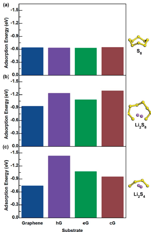
Fig. 3 Adsorption values of (a) S_8 , (b) Li_2S_8 , and (c) Li_2S_4 interacting with graphene, hG, eG and cG.
