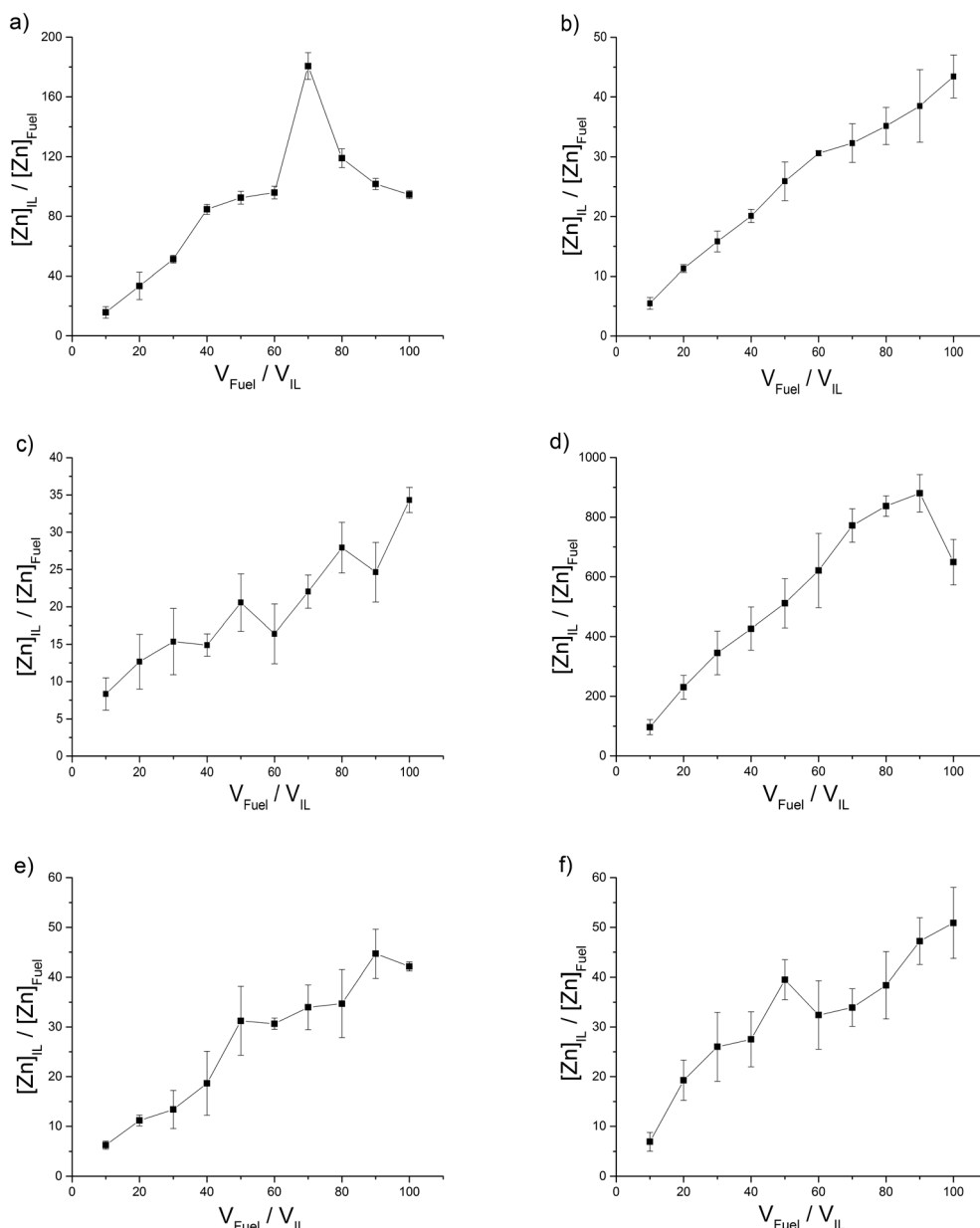
Fig. 4 ILs with a low distribution (L) of \text{Zn}^{2+} into the IL phase, (a) [C_4C_1\text{im}][\text{MeSO}_4] , (b) [C_4C_1\text{im}][\text{OTf}] (c) [C_4C_1\text{pyrr}][\text{OTf}] , (d) [C_8C_1\text{im}][\text{OTf}] and (e) [C_4C_1\text{im}][\text{N}(\text{Tf})_2] (f) [C_4C_1\text{pyrr}][\text{N}(\text{Tf})_2] .
