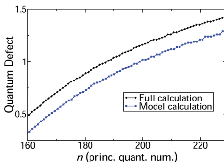
Fig. 4 Quantum defects for J = 0 HR states in the range n = 160 – 230 calculated using the full log derivative/MQDT approach outlined in the article, as well as a simple diabatic model (see text for details). The model calculations follow the trend for the full calculation closely.
