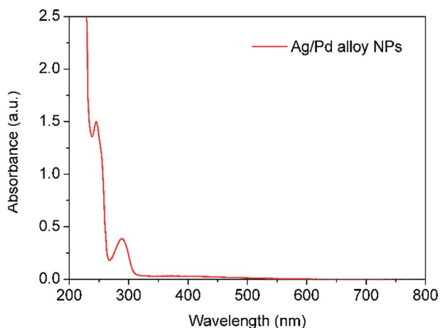
Fig. 12 UV-vis spectrum of Ag-Pd alloy NPs synthesized by simultaneous reduction of Ag(NO 3 ) and Pd(NO 3 ) 2 with HQ. The solution was diluted for 10 times prior to characterisation.
