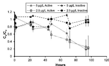
Fig. 4 Metaldehyde removal with active and inactive sand at 0.0025 and 0.005 mg L -1 ; error bars represent \pm 1 propagated error term (sum of root squared error terms for C_e and C_0 ).
