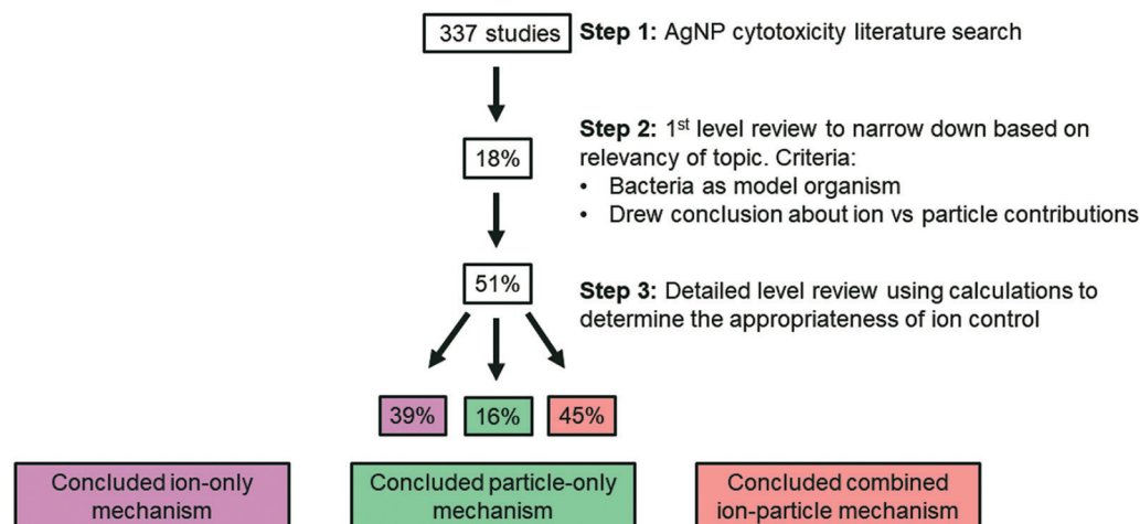
Fig. 3 Scheme of the literature review process. The percentage in the box is equal to the percentage of studies fulfilling the requirement for that particular step. Only 30 studies (51%) included a scaled ion control. Of those studies, 39% concluded an ion-only mechanism (stating that the particle does not play a role), while 16% and 45% concluded a particle-only or combined ion-particle mechanism (stating that the particle plays a role), respectively.
