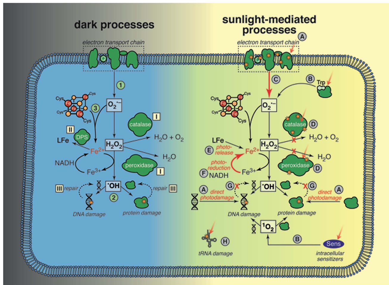
Fig. 7 Processes related to oxidative stress in bacteria: (1) Production of ROS. (2) Fenton damage to DNA and proteins. (3) Release of Fe from Fe-S proteins by O_2^{\cdot -} . Responses to mitigate oxidative stress: (I) enzymes scavenge ROS. (II) Sequestering of Fe. (III) Repair of damaged DNA and proteins. Mechanisms of damage by sunlight: (A) direct damage to DNA and proteins (membrane-bound or cytoplasmic). (B) Production of ROS by endogenous sensitizers. (C) Increased ROS production by damaged electron transport chain (ETC). (D) Damage to ROS scavenging enzymes. (E) Release of Fe. (F) Reduction of Fe(III) either by photons or by reducing equivalents. (G) Slowed repair of damaged DNA and proteins. (H) Direct damage to tRNA.
