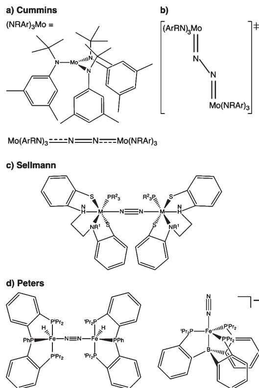
Fig. 2 Thermal dinitrogen activation complexes: (a) Cummins, (b) zig-zag transition state relevant to the Cummins complex, (c) Sellmann, (d) Peters: left [P_2^{PPh}FeH](\mu-N_2) , right [P_3^{BPh}Fe(N_2)]^- .
