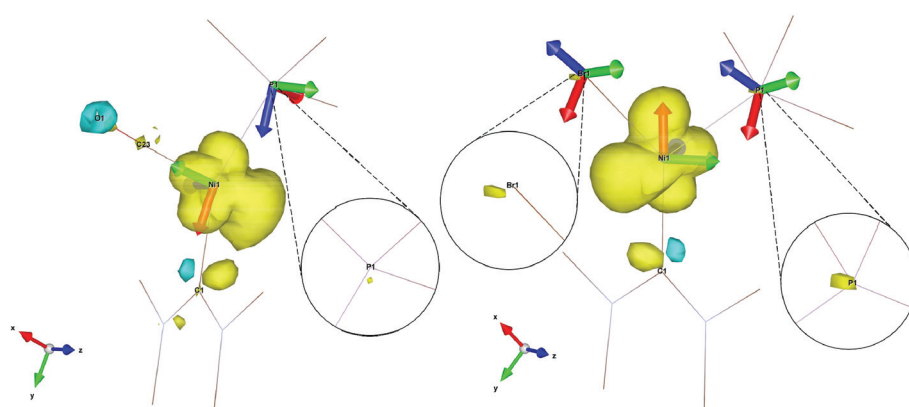
Fig. 11 Spin density contour plot with g - and A -frames for [\text{Ni}(\text{6-Mes})(\text{PPh}_3)(\text{CO})][\text{PF}_6] ( 5 , left) and [\text{Ni}(\text{6-Mes})(\text{PPh}_3)\text{Br}] ( 1 , right). Ligands are truncated for clarity.
