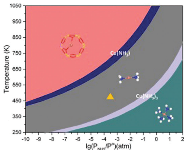
Fig. 7 Phase diagram for \text{Cu}(\text{NH}_3)_x in CHA with varying \text{NH}_3 pressure and temperature. The yellow triangle indicates typical operating conditions, i.e. a temperature of 473 K and an \text{NH}_3 concentration of 300 ppm. The phase-diagram is constructed with \text{NH}_3 in the gas-phase as reference. Reprinted with permission from ref. 164. Copyright 2018 The Royal Society of Chemistry.
