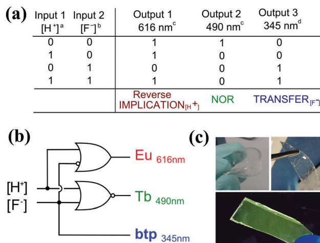
Fig. 24 (a) The truth table of the logic functions. a [H^+] = 2 mM; b [F^-] = 1 mM. (b) A circuit diagram of the observed logic gate functions. c Phosphorescence. d Fluorescence. (c) Images of Eu 1 and Tb 2 based gels when swelled in H 2 O (left) and CH 3 OH (right) under ambient light, after drying and irradiation at 254 nm, demonstrating the (0,0) state. Reproduced with small alterations from ref. 45 with permission from Royal Society of Chemistry, copyright 2015.
