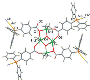
Fig. 2 Molecular structure of H-shaped heterometallic 2 . Colour scheme: tin, green; gold, yellow; phosphorous, orange; carbon, grey; oxygen, red; chlorine, purple; hydrogen, dark brown.
