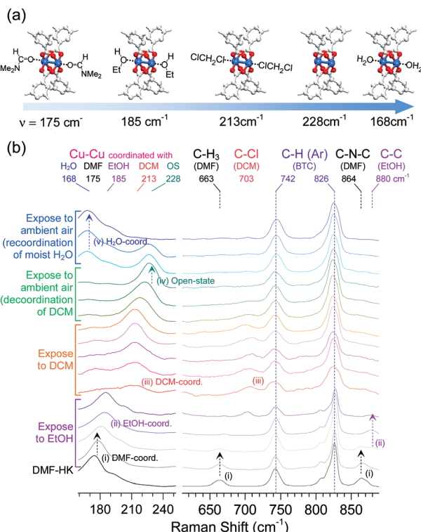
Fig. 11 (a) Illustrations of DMF-coordinated, EtOH-coordinated, DCM-coordinated, open-state, and H 2 O-coordinated ( \text{Cu}^{\text{II}}_2 ) centers in HKUST-1 (from left to right). (b) Successive changes of the in situ Raman spectra of DMF-coordinated HKUST-1 during sequential exposure to EtOH, DCM, and ambient air. Reprinted (adapted) with permission from ref. 69. Copyright (2017) American Chemical Society.
