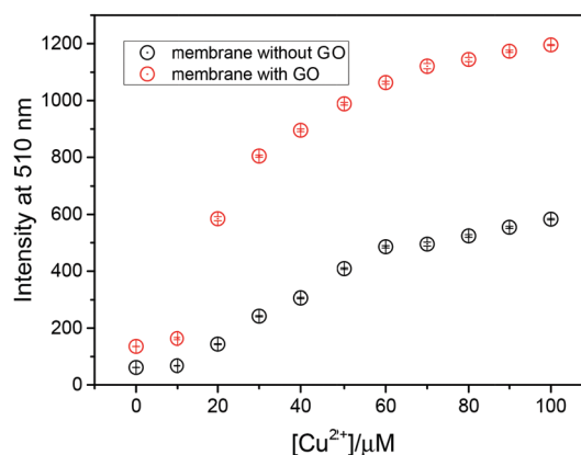
Fig. 2 Fluorescence intensity at 510 nm ( \lambda_{\text{ex}} = 410 nm) of probe 1 attached to the cellulose membrane with and without a GO coating.
