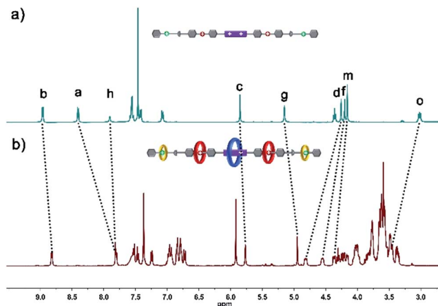
Fig. 3 Partial ^1\text{H} NMR spectra (400 MHz, 298 K, \text{CD}_3\text{CN} ) of (a) compound C1 and (b) hetero[6]rotaxane 8 .
