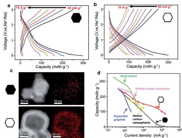
Fig. 5 Galvanostatic charge/discharge curves of (a) the non-hollow carbon nanoparticles and (b) the hollow carbon nanobubbles between 0.001 and 3.000 V (vs. \text{Na}^+/\text{Na} ) at various current densities, ranging from 50 to 15 000 \text{mA g}^{-1} . (c) Elemental mapping of sodium content in the non-hollow nanoparticles and the hollow nanobubbles after insertion of \text{Na}^+ ions at a current density of 10 000 \text{mA g}^{-1} . The red pixels represent sodium. (d) Rate capability for hard carbon, 42 expanded graphite, 11 hollow carbon nanowires, 41 hollow carbon nanospheres, 44 and our non-hollow carbon nanoparticles and hollow carbon nanobubbles.
