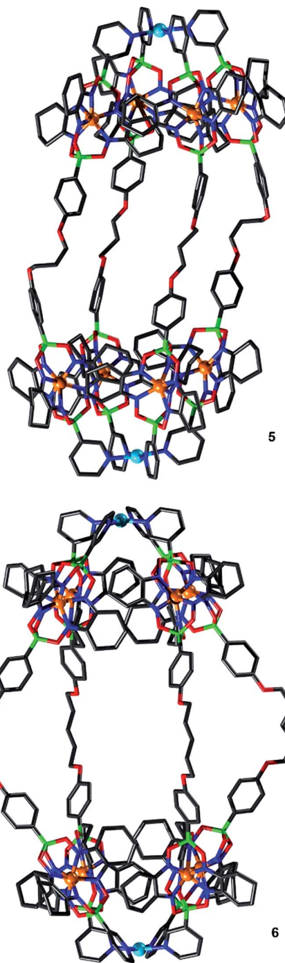
Fig. 6 Molecular structures of the cages 5 (top) and 6 (bottom) as determined by single crystal X-ray diffraction. Hydrogen atoms, solvent molecules and anions are omitted for clarity. Grey: C; dark blue: N; green: B; red: O; light blue: Pd and orange: Fe.
