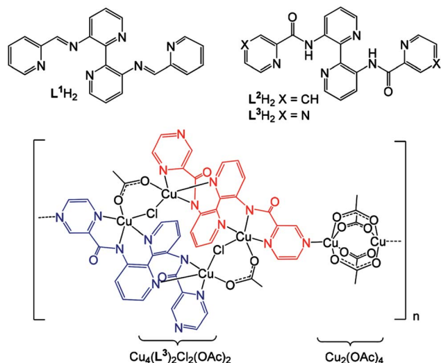
Fig. 13 (Top) Heterocyclic bis-imine and bis-amide ligands prepared from 3,3'-diamino-bpy. (Bottom) The molecular structure of CP comprised of a 1D arrangement of [Cu_4L_2Cl_2(OAc)_2] and paddle wheel [Cu_2(OAc)_4] units; for ease, the two ligands within the Cu_4 unit are shown in red and blue. [Reproduced from ref. 140 with permission from The Royal Society of Chemistry.]
