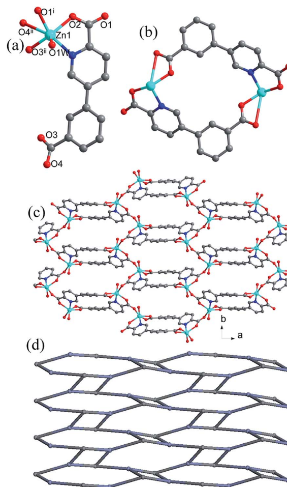
Fig. 1 (a) The coordination environment of Zn center, (b) the [\text{Zn}(\text{cppca})_2]_2 unit, (c) the 2D abnormal puckered layer, and (d) the topology structure in compound 1 .
