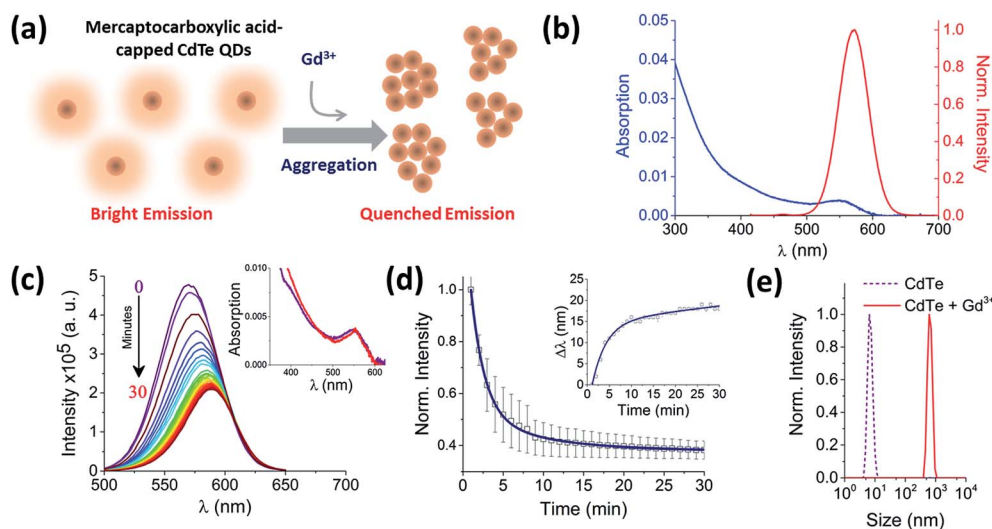
Fig. 1 Real-time probing of CdTe 580 QD aggregation induced by Gd 3+ . (a) The injection of a trivalent metal nitrate solution (10 \mu M Gd 3+ ) alters the ensemble fluorescence emission properties of 25 nM CdTe 580 (pH 8) as aggregation occurs. (b) Absorption (blue) and fluorescence emission spectrum with \lambda_{\text{exc}} = 400 nm (red) of 25 nM CdTe 580 QDs at pH 8. (c) Representative fluorescence quenching of 25 nM CdTe 580 QDs induced to aggregate over 30 minutes by addition of 10 \mu M Gd 3+ . Inset: variation in absorption spectra between the start ( t = 0 min, purple) and end ( t = 30 min, red) of the aggregation process. (d) The corresponding variation in fluorescence intensity and red shift (inset) across the 30 minute time window are shown. (e) DLS size distributions of CdTe 580 QDs prior to the injection of 10 \mu M Gd 3+ and at the endpoint ( t = 30 min) of the aggregation process.
