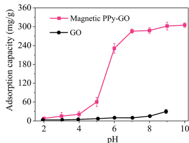
Fig. 8 Adsorption capacities of GO and magnetic PPy-GO under various pH conditions. Conditions: T = 300 K, RSL = 0.05 \text{ g L}^{-1} and C_0 = 20 \text{ mg L}^{-1} for magnetic PPy-GO; T = 298 K, RSL = 0.5 \text{ g L}^{-1} and C_0 = 100 \text{ mg L}^{-1} for GO. 32
