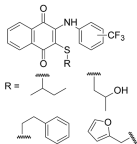
Fig. 3 Structures of the sulfanyl derivatives of 1,4-naphthoquinone based on aryl amines containing -CF_3 group.
