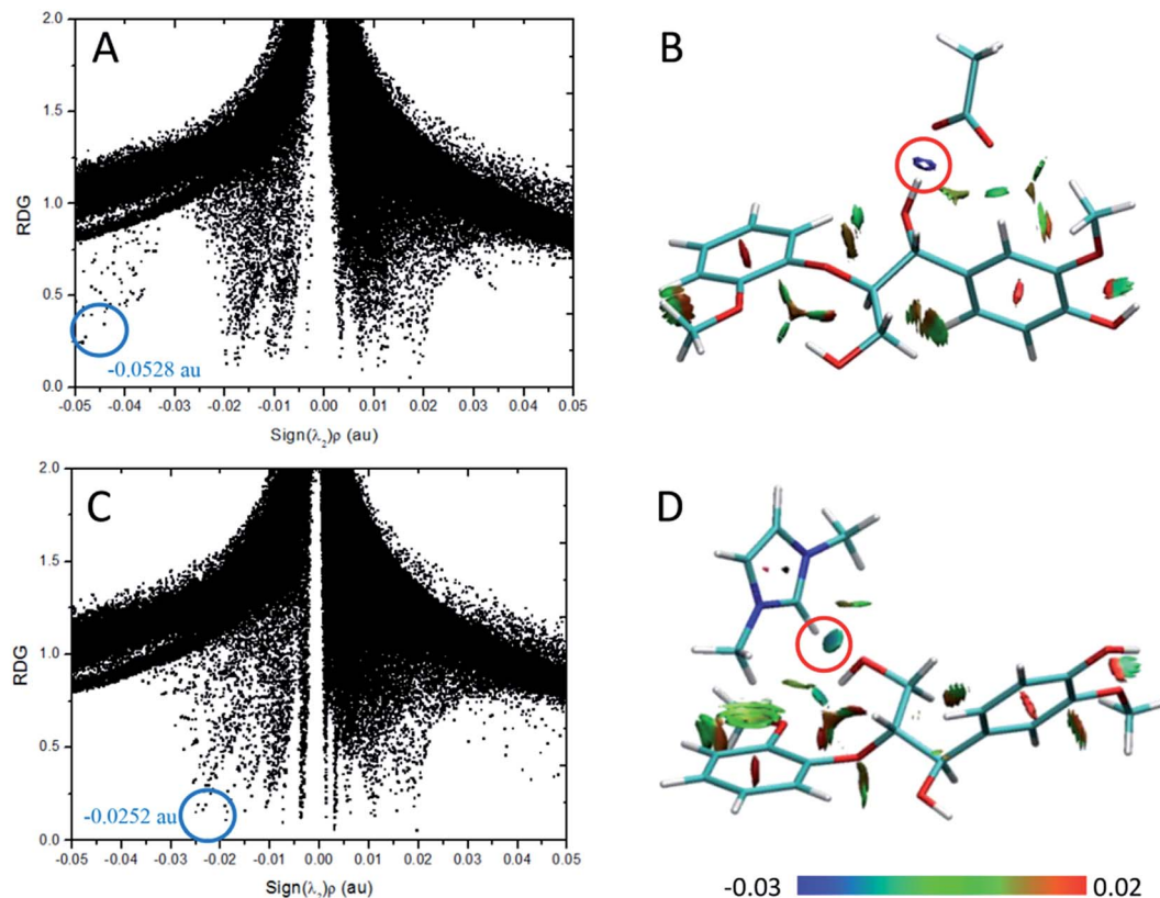
Fig. 2 RDG scatter plots (isovalue = 0.5 a.u.) and surface plots ( s = 0.7 \text{ a.u.} ) of (A and B) OAc–GG interaction and (C and D) Mmim–GG interaction. The isosurfaces are colored on a blue–green–red scale according to values of \text{sign}(\lambda_2)\rho , ranging from -0.03 to 0.02 \text{ a.u.} Blue indicates strong attractive interactions and green indicates the \pi -stacking interaction.
