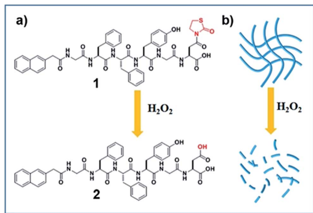
Scheme 1 (a) Chemical structures of Nap-GFFYGD(Thi) (compound 1 ) and Nap-GFFYGD (compound 2 ) and H 2 O 2 triggered conversion. (b) Schematic representation of possible H 2 O 2 triggered hydrogel degradation.
