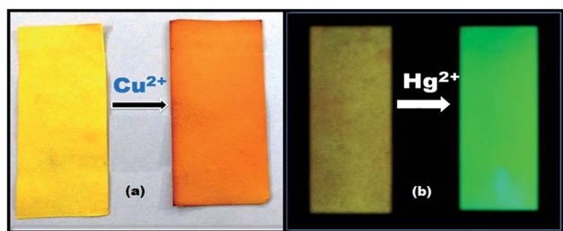
Fig. 11 (a) Naked eye detection on a piece of paper soaked with FDNS: from left to right FDNS (blank); FDNS + Cu 2+ (b) the variation of the color of FDNS coated on filter paper before (left) and after treatment with Hg 2+ (right) under UV excitation light.
