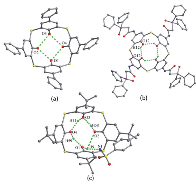
2.2 O-Monosubstituted thiacalix[4]arenes
