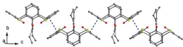
Fig. 17 An infinite chain of 22 built by \pi - \pi stacking.
