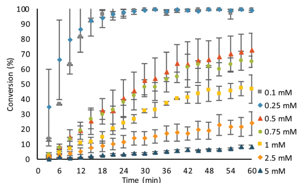
Fig. 2 Conversion of the substrate 1 to the product after addition of \beta -Gal (1 U mL -1 ) using different concentrations of the substrate at room temperature in Tris buffer (pH 7, 50 mM). Error bars represent the standard deviation where n = 3 .
