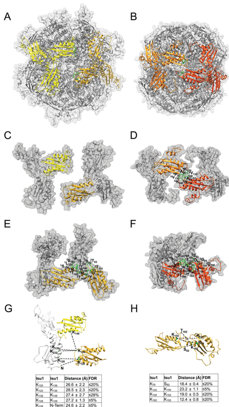
Fig. 7 Proposed [2Fe-2S] cluster assembly site of the [Yfh1]_{24} \cdot [Isu1]_{24}^{LMW} complex. (A) Top view of two Fe-S cluster assembly sites formed by two adjacent [Yfh1]_3 \cdot [Isu1]_{12}^{LMW} sub-complexes at the 2-fold axis of the [Yfh1]_{24} \cdot [Isu1]_{24}^{LMW} complex. Isu1 trimers are shown as yellow and gold ribbons with Fe-S cluster coordinating residues shown as green sticks. (B) The 2-fold axis of the [Yfh1]_{24} \cdot [Isu1]_{24}^{HWM} complex, with Isu1 trimers shown as light orange and orange ribbons, is shown for a comparison. 16 (C) In the [Yfh1]_{24} \cdot [Isu1]_{24}^{LMW} complex, the PISA program did not identify any interfaces between the two adjacent Isu1 trimers at the 2-fold axis; (D) PISA otherwise identified one interface between the two adjacent Isu1 trimers in the [Yfh1]_{24} \cdot [Isu1]_{24}^{HWM} complex. 16 Conserved residues within this interface, predicted to form hydrophobic interactions, are shown as green sticks (see also Table 5 for additional details). The letters a and b denote the two adjacent Isu1 trimers. (E) In the [Yfh1]_{24} \cdot [Isu1]_{24}^{LMW} complex, the PISA program identified an interface between two subunits of the same Isu1 trimer around the 3-fold axis. Residues within this interface, predicted to form hydrogen bonds and salt bridges between the two proteins, are shown as green sticks. The numbers 1 and 2 denote different subunits of the same Isu1 trimer. (F) As in (E) for the [Yfh1]_{24} \cdot [Isu1]_{24}^{HWM} complex 16 (see also Table 5 for additional details). (G) The interface shown in (C) fulfills the distance constraints or maximum allowable distance constraints set by the Isu1-Isu1 cross-links shown. (H) The interface shown in (E) fulfills the distance constraints set by the Isu1-Isu1 cross-links shown. The table underneath each structure provides the distances between each pair of cross-linked residues shown in the structure, and the False Discovery Rate (FDR) of the corresponding cross-linked peptides. See Table S1 (ESI†) for additional details.
