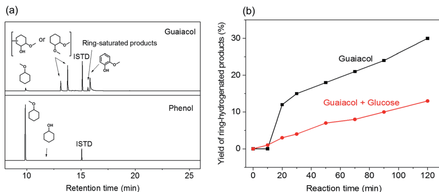
Fig. 5 (a) Gas chromatograms of the reactions in methanol using phenol and guaiacol as model substrates; (b) yield of ring-hydrogenated products obtained from the hydrogenation reaction of guaiacol (black) and guaiacol + glucose (red) in methanol (conditions: 50 mg of substrate, 30 ml of methanol, 10 mg of Pd/C, 160 °C, 2 h, 30 bar H 2 ).
