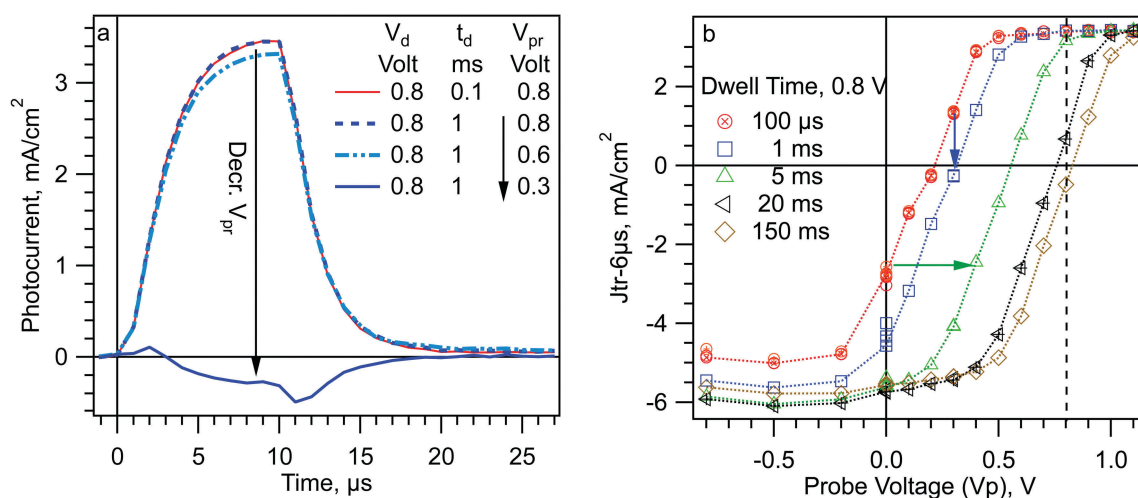
Fig. 4 Results of SDSP experiments on a planar MAPI cell. (a) Example photocurrent transients for a dwell voltage ( V_d ) of 0.8 \text{ V} . (b) J_{\text{tr}}-6\mu\text{s} vs. V_{\text{pr}} and t_d , from SDSP experiments using a dwell voltage of 0.8 \text{ V} .
