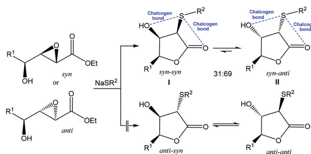
Scheme 3 Chalcogen bond assisted stereoselective synthesis of lactones. 62
