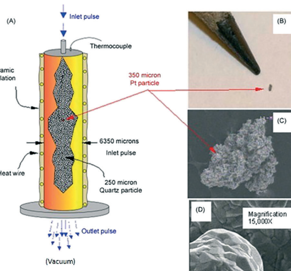
Fig. 9 A) Schematic of TAP microreactor single particle configuration. (B) Actual image of single particle Pt polycrystalline catalyst taken with a digital camera. (C) SEM images showing the entire polycrystalline Pt particle. (D) Inset gives high magnification (15 000×) SEM image of Pt particle surface. 18
