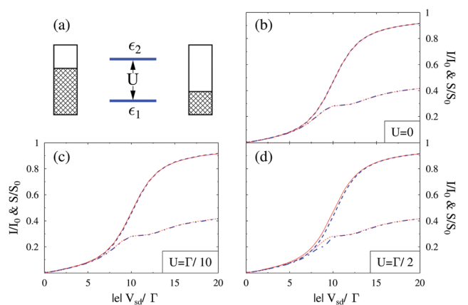
Fig. 13 Full counting statistics of electron transport in junctions. Simulation is performed for Hubbard model (a), \hat{H}_M = \sum_{i=1,2} \epsilon_i \hat{n}_i + U \hat{n}_1 \hat{n}_2 ,
