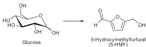
Scheme 4 Conversion of glucose to 5-HMF.
