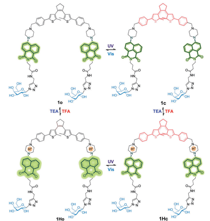
Scheme 1 Structural transformations of 1o in response to UV/Vis and TFA/TEA stimuli.
