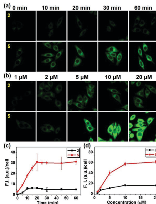
Fig. 1 Confocal microscopy images of HeLa cells upon treatment with probes 2 and 5 . (a) The fluorescent images were obtained at variable time (2 \mu M each); (b) and at variable probe's concentration for 10 min. The cells were incubated in high glucose serum free DMEM media at 37 ^{\circ} C, \lambda_{\text{ex}} = 458 nm, bandpass filter (505–550 nm). (c and d) Fluorescence intensities (a.u.) per cell in the images of the panel (a) and (b) respectively. The images were obtained using Image J software. The data are presented as mean \pm SD ( n = 5).
