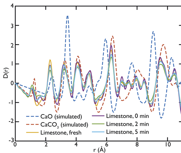
Fig. 9 Comparison of the experimental Ag-anode X-ray PDFs of the limestone series with the calculated PDFs. Most features of the experimental data are well represented by the \text{CaCO}_3 model, confirming that this is the main phase present in this series of samples.
