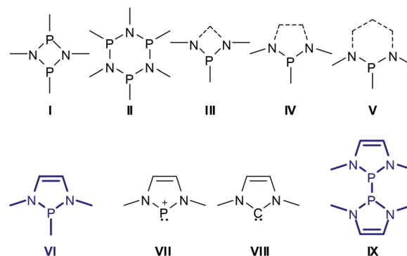
Scheme 1 Molecular structures of generic phosphazanes ( I , II ) and organic N-heterocyclic phosphines covered in this review ( VI , IX ), and phosphonium ions derived from these by abstraction of a P-substituent ( VII ). Dashed lines may be single or double bonds.
